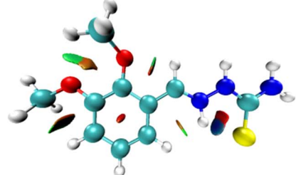
Fig. 13 The RDG scatter plots (upper) and NCI plots (bottom) isosurface ( s = 0.5 a.u.) of the neutral (a) and protonated structures (b and c) of DMPTS, as well as the color map and chemical explanation (d).
