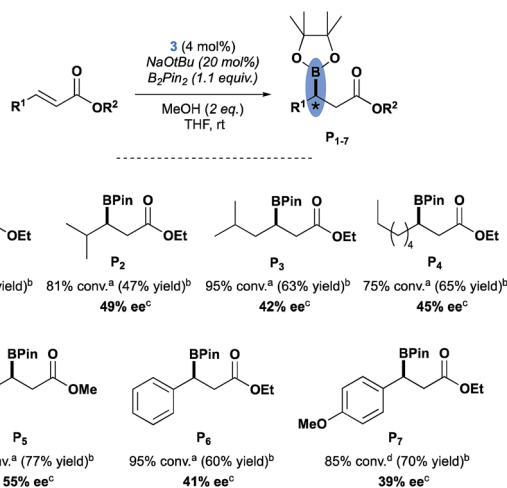
Scheme 7 Evaluation of Cholest t CAACuCl complex 3 in ACB reaction. a Determined by 1 H NMR spectroscopy using mesitylene as an internal standard. b Isolated yield after SiO 2 purification. c Determined by GC on a chiral stationary phase (see ESI for details † ). d Anthracene was used as internal standard.
