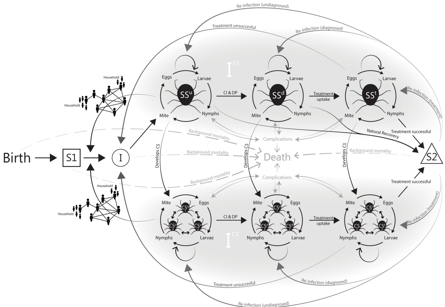
Fig 2. Scabies transmission model. Abbreviations: CI & DP, case identification and diagnostic processes; CSd, crusted scabies diagnosed; CSu, crusted scabies undiagnosed; CSu, crusted scabies treatment; I, infectious; R, recovered; S1, susceptible (never has been scabies infected); S2, susceptible (after prior scabies infection); SSd, simple scabies diagnosed; SSu, simple scabies undiagnosed; SSu, simple scabies treatment. The figure shows a susceptible population (S1) of individuals who can be infected (I) with scabies. The probability of infection depends on the interaction between individuals with other, infected, members of their household or community reflected by the network diagrams. Infected patients develop simple scabies (ISS), which is initially undiagnosed (SSu). Case identification and diagnostic processes (CI & DP) determine the probability that a patient becomes diagnosed (SSd). Subsequently, there is a probability that a patient takes up treatment and moves to SS t . Treatment has a probability of success, dependent on treatment efficacy and compliance. In this case, patients are cured and susceptible for reinfection (S2), the probability and infectiousness of which can differ from the probability and infectiousness in individuals who never had scabies before. Re-infection or sustained infection after unsuccessful treatment can go undiagnosed if a patient does not receive appropriate follow-up. A proportion of patients with simple scabies will develop CS. Grade 1 CS (CS1) can progress to grade 2 CS (CS2) and grade 3 CS (CS3). While both simple scabies and CS can result in complications, the probability of this is higher in patients with CS and increases with higher grade CS. Complications can result in death or can resolve. “Background mortality” reflects people who die from other causes than CS, which can differ between the susceptible and infected populations due to differences in comorbidities. In case the model is used to inform an economic evaluation, each of the health states (S1, SSu, SSd, SS t , CSu (grades 1–3), CSd (grades 1–3), CS t (grades 1–3) and S2) is associated with a cost and a utility. Diagnostics, treatments and complications can be associated with additional costs and/or (dis)utilities. The model can be used to simulate a community and how individuals move through the various health states over time, accruing costs, life-years and utility based on the time they spend in each of the health states. Results can be expressed in terms of costs per quality-adjusted life year (QALY) gained, or any other outcome captured in the model (e.g. cost per reinfection prevented or cost per life year gained).
