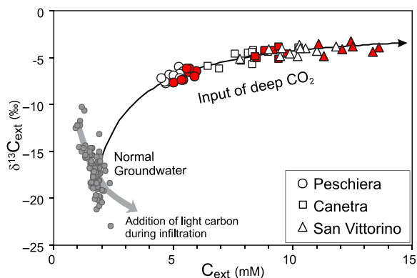
Fig. 3. CO 2 sources and dissolved carbon in the monitored springs. \delta^{13}C_{ext} versus C_{ext} diagram of the monitored springs from the Velino aquifer. Measurements are compared with the theoretical compositions obtained adding a deep inorganic CO 2 ( \delta^{13}C = -1.48\text{‰} ) to normal groundwaters. Samples taken in periods close to the main earthquakes (red symbols) show evident shifts toward the same deep CO 2 component (i.e., of similar isotopic carbon signature) that enter the aquifer during the quiescence periods (white symbols).
