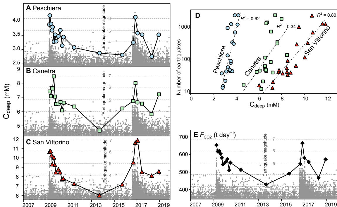
Fig. 2. Temporal evolution of CO 2 degassing and seismicity. (A to C) Chronograms of the earthquake magnitudes compared with the concentration of deeply derived carbon ( C_{deep} ) in the monitored springs. (D) Binary plots of C_{deep} of the monitored springs against the log number of the earthquakes occurred at distances <45 km in a period of 80 days centered at any sampling date. (E) Chronogram of the earthquake magnitudes compared with the daily amount of deeply derived CO 2 dissolved by the groundwaters of the Velino aquifer ( F_{CO_2} ).
