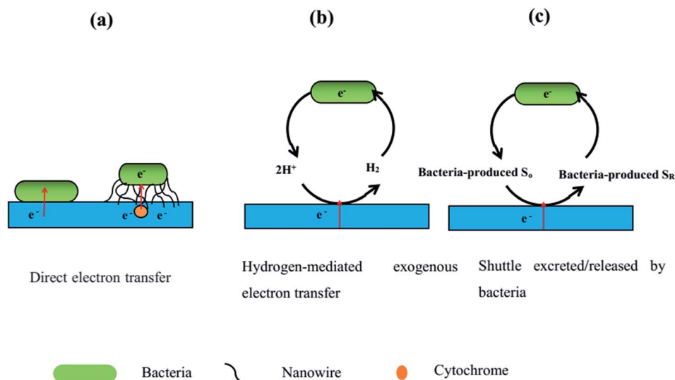
Fig. 7 The three possible ways of extracellular electron transfer mechanisms from the cathode to the microbial catalysts. S_O is oxidized electron shuttle and S_R is reduced electron shuttle.
