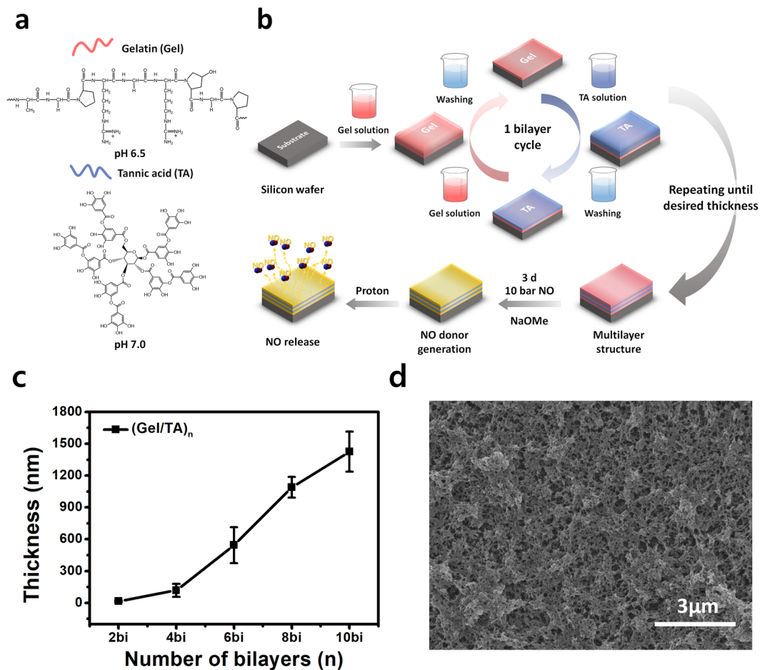
Figure 1. (a) Molecular structure and pH condition of film combination and (b) schematic illustration about preparation method of gelatin/tannic acid multilayer film for controlled nitric oxide release (c) film growth curve measured by profilometry and (d) scanning electron microscopy image of 10-bilayer film (Fig. 1 schematic illustration was drawn by K.P.).
