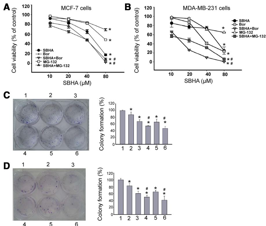
Figure 1 Effects of combined treatment with SBHA and proteasome inhibitors on breast cancer cell growth. (A) MCF-7 and (B) MDA-MB-231 cells were treated with SBHA, Bortezomib, and MG-132 alone or in combination for 72 h and cell proliferation was assessed using the WST-8 assay. The concentration of Bortezomib and MG-132 was 8000- and 160-fold times that of SBHA, respectively. The proliferation of untreated control cells was considered as 100%. * P < 0.05 vs. control; # P < 0.05 vs. each reagent alone. (C) MCF-7 and (D) MDA-MB-231 cells were exposed to SBHA (40 μM), Bortezomib (5 nM), and MG-132 (250 nM), alone or in combination, for 72 h and plated onto 6-well plates at a density of 500 cells per well. Colonies were numbered after 14-day incubation. Left panel: Representative dishes of cells of each group stained with Giemsa. Right panel: Quantitation of colony formation. Colony formation rate was calculated as percentage of total seeded cells. 1-6: control, SBHA, Bortezomib, SBHA + Bortezomib, MG-132, and SBHA + MG-132 group, respectively. * P < 0.05 vs. control; # P < 0.05 vs. SBHA alone.
