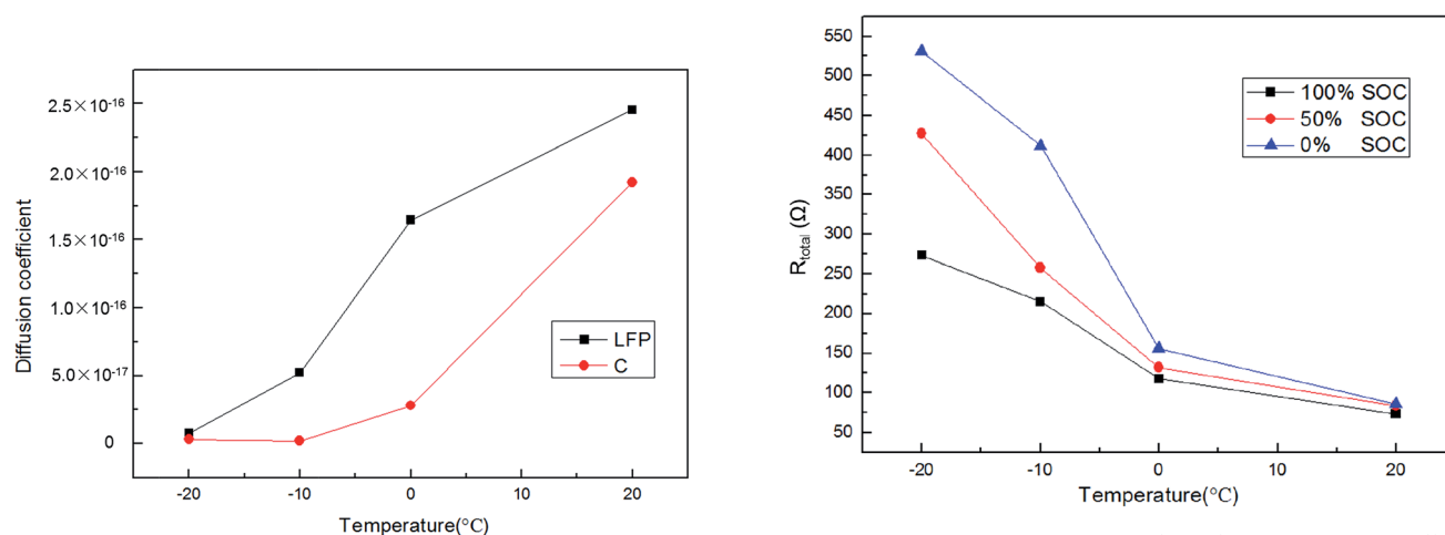
Fig. 9 The total internal resistance of the fabricated cell at different temperatures (20 °C, 0 °C, -10 °C and -20 °C) and different SOCs (0%, 50% and 100%).
