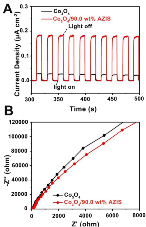
Fig. 7 (A) The transient photocurrent density curves and (B) the EIS Nyquist plots of \text{Co}_3\text{O}_4 and \text{Co}_3\text{O}_4/90.0 wt% AZIS.
