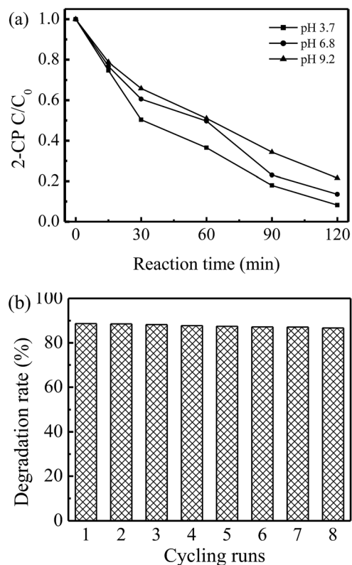
Fig. 11 (a) Degradation of 2-CP in rGO-4-PPNc Fenton-like systems under different pH conditions. (b) Reusability of rGO-4-PP Nc for 2-CP degradation at neutral conditions.
