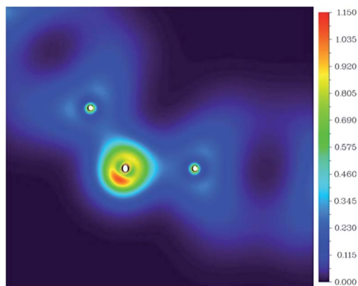
Fig. 3 The two-dimensional valence-electron density color-filled map of rGO-4-PP Nc in the C1–O1–C2 plane. The length unit is Angstrom.
