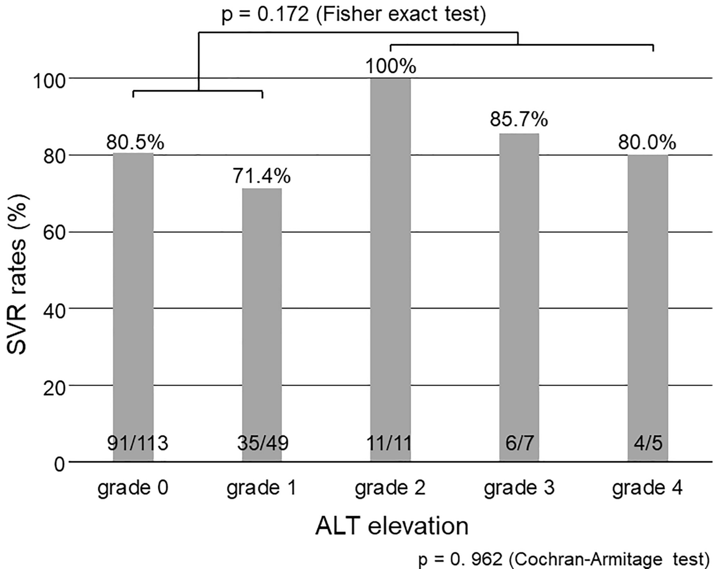
Fig 1. SVR rates according to the grade classification for ALT elevation. There is no significant association between grades of ALT elevation and SVR rates ( p = 0.962 by Cochran–Armitage test for trends). The SVR rates in patients with grades 2–4 ALT elevation are numerically higher than those in patients with grades 0–1, although there is no significant difference ( p = 0.172 by Fisher’s exact test). SVR, sustained virological response; ALT, alanine aminotransferase.
