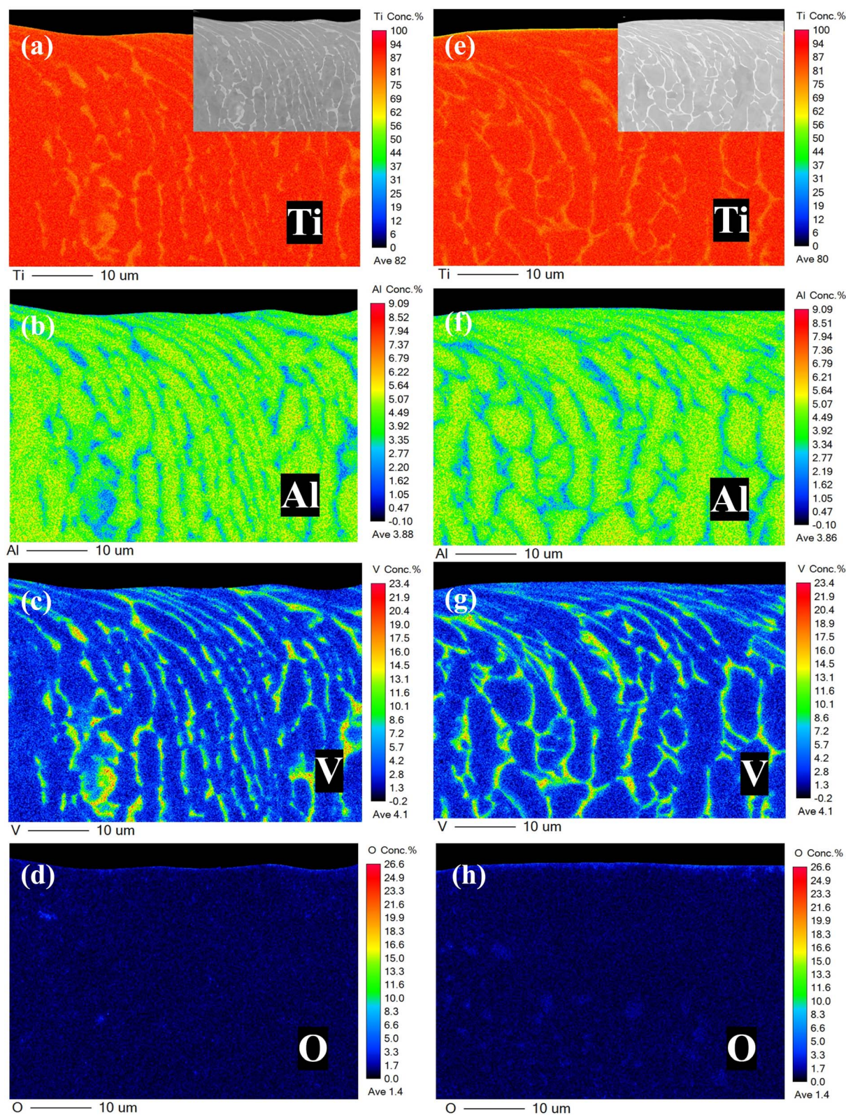
Fig. 7 Wear scar section under different DOCs: (a–d) element distributions of Ti, Al, V, O in the wear scar section under high DOC, (e–h) element distributions of Ti, Al, V, O in the wear scar section under low DOC.
