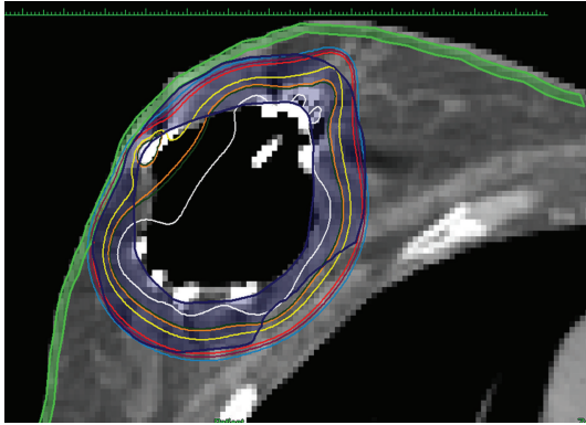
FIGURE 7: SAVI 10-1 implant. Notice how the isodose lines pull away from the skin surface. The maximum dose to a 0.1 cc volume of skin is 101% of the prescribed 34 Gy. The maximum dose to a 0.1 cc volume of rib is 100% of the prescribed 34 Gy. There is excellent dosimetric coverage of the PTV_EVAL (V95 = 96% with only 0.9% nonconformance).
