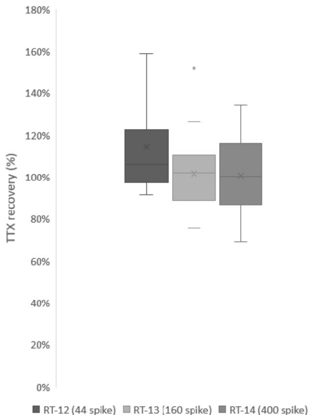
Figure 1. Box and whisker plot illustrating variability of TTX recoveries determined across all participants from spiked mussel samples, RT12 (44 \mu\text{g}/\text{kg} ), RT13 (160 \mu\text{g}/\text{kg} ), and RT14 (400 \mu\text{g}/\text{kg} ).
