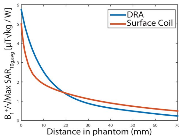
FIG. 6. Simulated B_1^+ profile normalized to maximum SAR_{10g, avg} for a dielectric resonator and loop coil placed on a phantom ( 120 \times 120 \times 210 mm 3 , \epsilon_r = 80 , \sigma = 0.40 S/m). DRA, dielectric resonator antenna; SAR, specific absorption rate.
