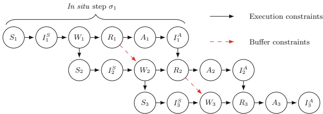
Fig. 3. Dependency constraints within and across in situ steps. (Color figure online)
