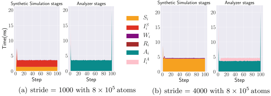
Fig. 6. Execution time per step for each component with a helper-core placement (all component on the same node). The Synthetic Simulation stages are on the left and the Analyzer stages are on the right (lower is better).
