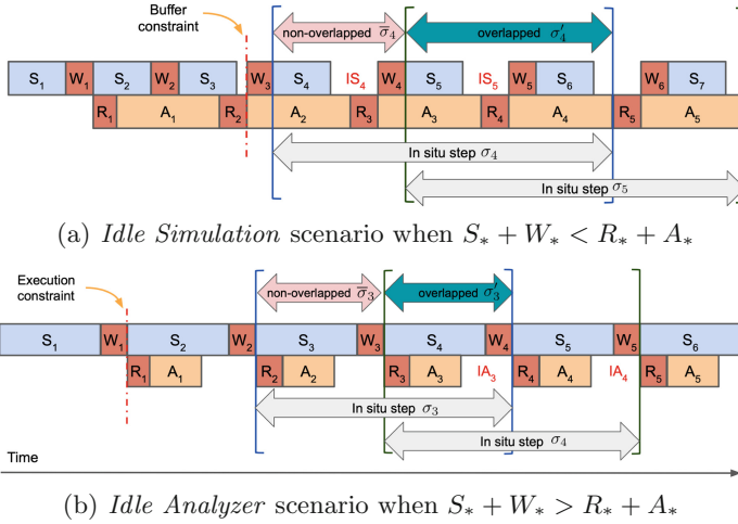
Fig. 2. Two different execution scenarios for in situ workflow execution.
