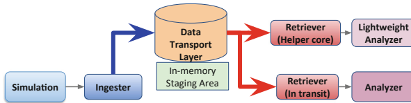
Fig. 1. A general in situ workflow software architecture.
