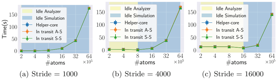
Fig. 7. Detailed idle time I_* for three component placements at different strides when varying the number of atoms (lower is better).
