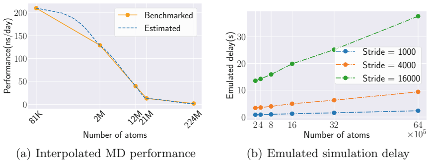
Fig. 5. MD benchmarking results from the literature obtained by using 512 NVIDIA K20X GPUs. The results are interpolated to obtain the (a) estimated performance and then combined with the stride to synthesize the (b) emulated simulation delay.
