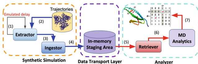
Fig. 4. Synthetic Workflow: the Extractor (1) sleeps during the emulated delay, then (2) extracts a snapshot of atomic states from existing trajectories and (3) stores it into a synthetic frame. The Ingestor (4) serializes the frame as a chunk and stages it in memory, then the Retriever (5) gets the chunk from the DTL and deserializes it into a frame.
