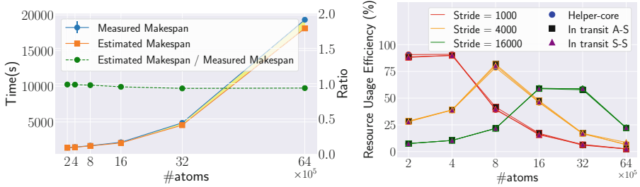
Fig. 8. Left: MAKESPAN is estimated from 100\bar{\sigma}_* using the helper-core component placement with stride 16000, the yellow region represents the error. Ratio of Estimated MAKESPAN to Measured MAKESPAN uses the second y-axes on the right (close to 1 is better). Right: Resource usage efficiency (higher is better). (Color figure online)
