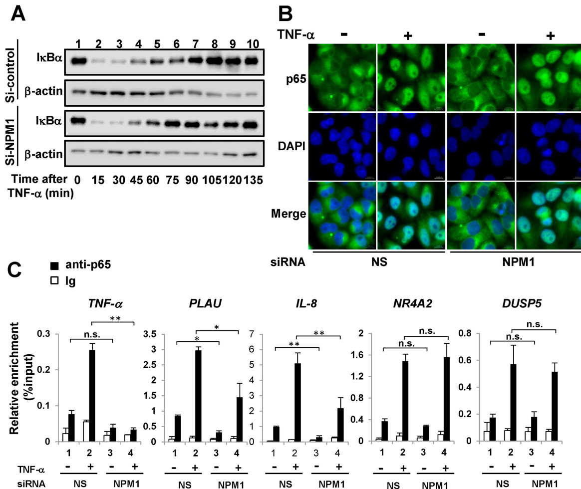
Figure 3. NPM1 regulates the target gene binding of NF- \kappa B, but not its nuclear translocation. (A) Effect of NPM1 knockdown on the expression level of I- \kappa B \alpha . The amounts of I- \kappa B \alpha and \beta -actin in HeLa cells treated with control siRNA or NPM1 siRNA after TNF- \alpha treatment were examined by western blotting. Time (min) after TNF- \alpha treatment is shown at the bottom of the panel. (B) Localization of p65 after TNF- \alpha treatment in HeLa cells treated with control or NPM1 siRNA. DNA was counter stained by DAPI. (C) Recruitment of p65 to its target genes. HeLa cells transfected with siRNAs as indicated were incubated without or with TNF- \alpha for 1 h, followed by ChIP assay. The precipitated DNA amounts containing the promoter regions of the genes listed in Figure 2D (TNF- \alpha , PLAU and IL-8 ) and those of stimulated genes ( NR4A2 and DUSP5 ) by NPM1 knockdown were quantitatively analyzed by q-PCR. Three independent experiments were performed and error bars indicates \pm SD. The results were statistically analyzed by student t -test and ***, ** and * indicate P < 0.001 , 0.01 and 0.05, respectively.
