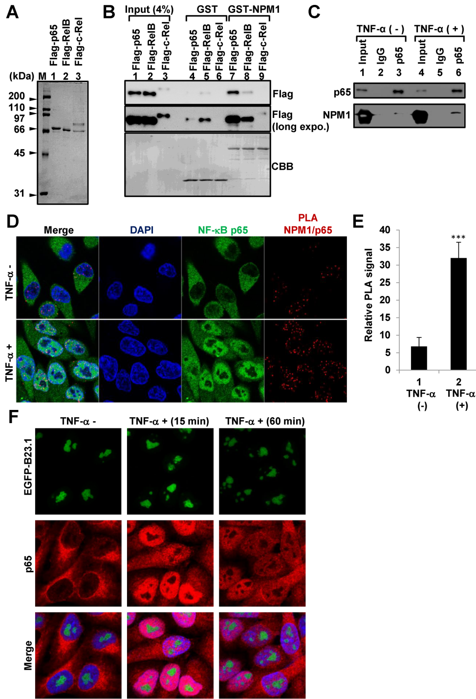
Figure 1. Interaction between NPM1 and NF-κB. (A) Purified NF-κB proteins. Flag tagged p65, RelB and c-Rel were expressed in 293T cells, purified with Flag-affinity gel, separated by 10% SDS-PAGE and visualized by CBB staining. (B) Direct interaction between NPM1 and the NF-κB proteins. GST pull-down assays using GST or GST-NPM1 (lanes 4–6 and 7–9) with purified Flag-p65 (RelA), -RelB or -c-Rel were performed. Flag-tagged NF-κB proteins were detected by western blotting and the GST proteins were visualized by CBB staining. (C) Immunoprecipitation assay. Cell extracts were prepared from HeLa cells treated without or with TNF-α for 30 min, and the interaction between NPM1 and p65 was analyzed by immunoprecipitation with control Ig and anti-p65 antibody. The input (lanes 1 and 4) and immunoprecipitated (lanes 2, 3, 5 and 6) proteins were separated by SDS-PAGE and analyzed by western blotting with anti-NPM1 and p65 antibodies. (D and E) In vivo interaction between NPM1 and p65. HeLa cells were treated with or without 20 ng/ml TNF-α for 1 h, in situ proximity ligation assays (PLAs) were performed using primary antibodies against NPM1 and p65. The PLA signals in panel C were quantitatively analyzed by the image processing software Imaris. The average spot number per cell was calculated from randomly selected cells ( n = 20 ). Error bars represent \pm SD, statistical significance was calculated using student's t -test and *** indicates P < 0.001 . (F) Localization of NPM1 in TNF-α treated cells. HeLa cells stably expressing EGFP-NPM1 were treated without or with TNF-α (20 ng/ml) for 15 min and 60 min, followed by immunofluorescence analysis with anti-p65 antibody and the localization of the proteins was observed by a confocal microscope. Bar at the bottom indicates 10 \mu m.
