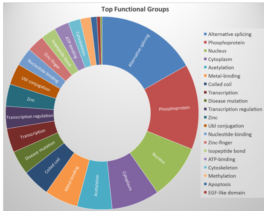
Fig. 2 Proportions of numbers of genes involved in the top 20 Uniprot functional groups
