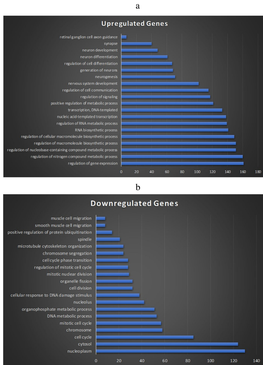
Fig. 3 Functional groups listed by the up- or down-regulated set and the numbers of genes involved in each function group. a , 20 top functions for upregulated groups and b , 20 top functions for down-regulated groups
