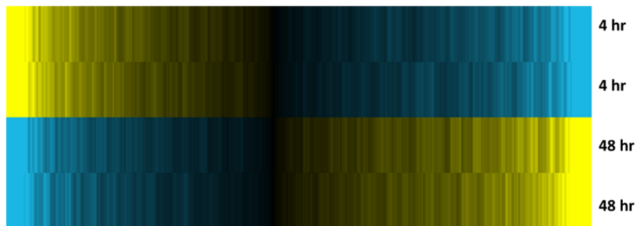
Fig. 1 Heat map presentation of the differentially expressed genes after BoNT/A 4 and 48-h treatment. The heat map includes 1368 probes after running the ANOVA analysis with unadjusted p -value < 0.01. The values are mean centered with yellow indicating higher expression and blue indicating lower expression. Compared to the 4-h treatment, the 48-h treatment induces 744 up-regulated and 624 down-regulated genes
