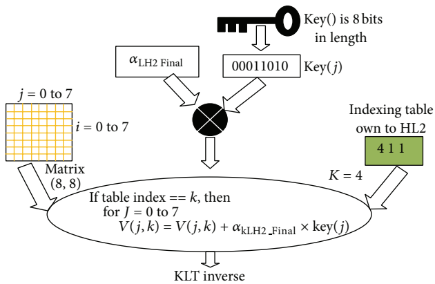
FIGURE 10: Insertion step in the matrix 8x8 applied on the Karhunen Loeve components.
