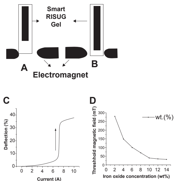
Figure 5 Response of Smart RISUG. A) No magnetic field. B) Electromagnet at the lower end caused Cuproferrogel elongation. C) Smart RISUG deflection \Delta h/h_0 (%) versus current (A) given –a hysteresis graph obtained (D) Threshold magnetic field vs iron oxide concentration. The presence of 10% iron oxide causes threshold magnetic field effect in presence of external magnetic field.
