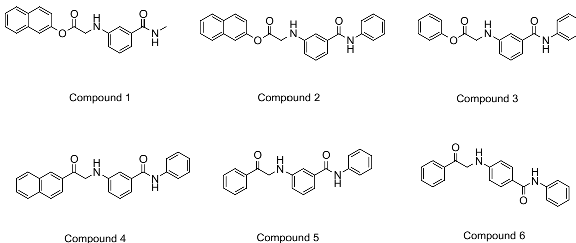
Figure 5 Chemical structures of compounds 1–6.
