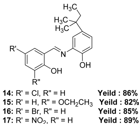
Fig. 15 Structure of Schiff base ligands 14, 15, 16 and 17.
