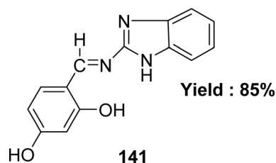
Fig. 59 Structure of Schiff base ligand 141 .
