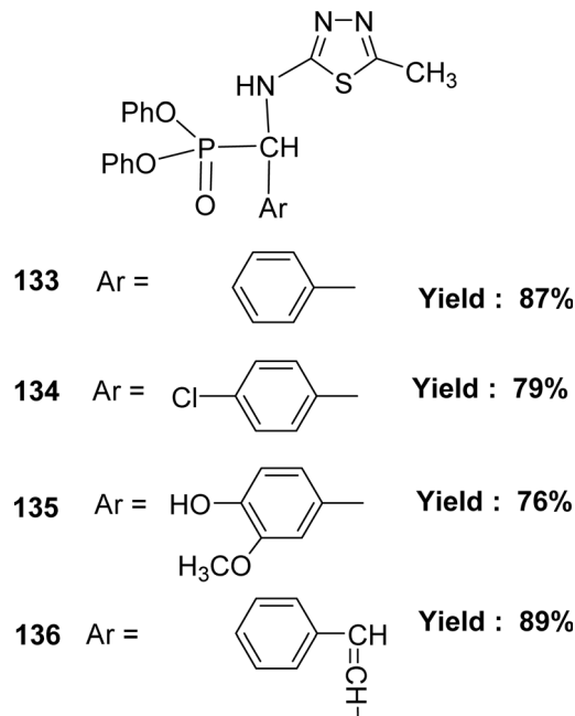
Fig. 54 Structure of compounds 133–136.
