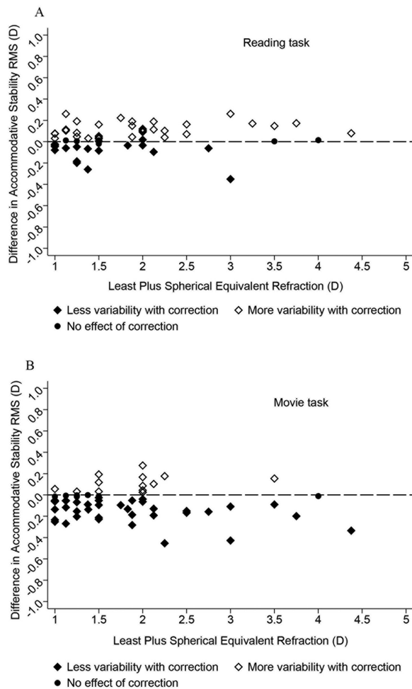
FIGURE 3. (A) Effect of hyperopic refractive correction on the stability of the accommodative response in the reading task, calculated as the difference between the root mean square error (RMSE) of the accommodative response with and without correction. (B) Effect of correction on the stability of the accommodative response in the movie task, calculated as the difference between the RMSE of the accommodative response with and without correction. The long-dashed line represents no effect of correction (difference of zero). Data points above long-dashed line represent more accommodative response instability with correction, while those below line represents less instability with correction.
