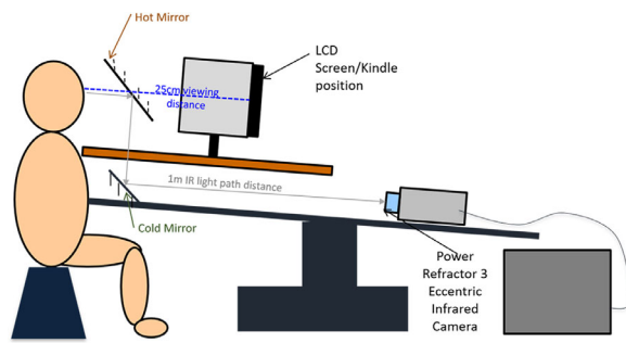
FIGURE 1. A schematic diagram of operation of the PowerRef 3 infrared photorefraction system, which used two periscopic hot/cold mirrors to reflect infrared light from the instrument's camera aperture into the eye, to enable the reading and movie tasks to be viewed directly on visual axis. The entire table was tilted by 16.7 degrees to enable participants to view in downgaze, thus adopting a more natural reading position.
