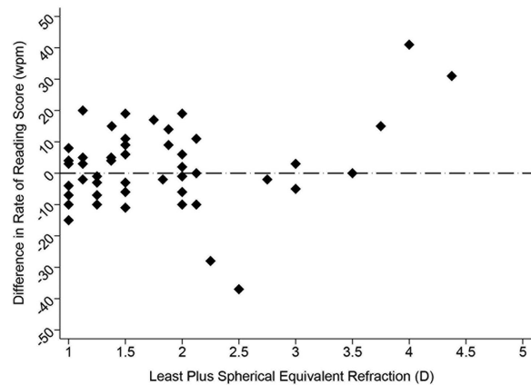
FIGURE 4. Improvement in reading speed with hyperopic refractive correction. This was calculated as the difference between the reading speed score with and without correction. Long-dashed line represents no effect of correction (difference of zero). Data points above line represent improvement in reading speed with correction.
