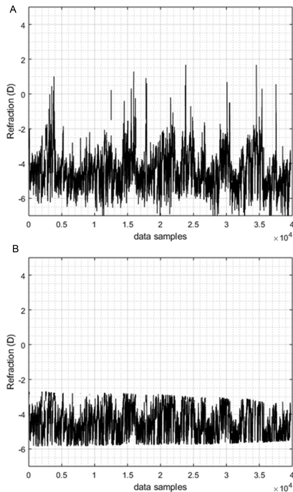
FIGURE 2. (A) An example of the accommodative response over time in the reading task showing apparent variation in response when participant was reading the top and bottom of the Kindle screen, in up and down-gaze positions. (B) The same accommodative response after data points corresponding to these outliers in panel A were removed. The Y-axis represents refraction (from which the accommodative response was computed), and the X-axis represents the length of the data samples (from which the duration of measurement can be derived, given the 50 Hz sampling frequency of the PowerRef 3).
