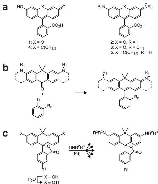
Figure 1. (a) Chemical structures of xanthenes and carbon-containing isologues. (b) Existing synthetic strategy to carborhodamine dyes. (c) Divergent synthesis of carborhodamines through carbofluorescein intermediates.
