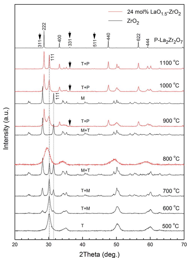
Fig. 3 XRD patterns of \text{ZrO}_2 and 24 mol% \text{LaO}_{1.5}\text{-ZrO}_2 powders after annealing at 500\text{--}1100 \text{ }^\circ\text{C} for 6 h.
