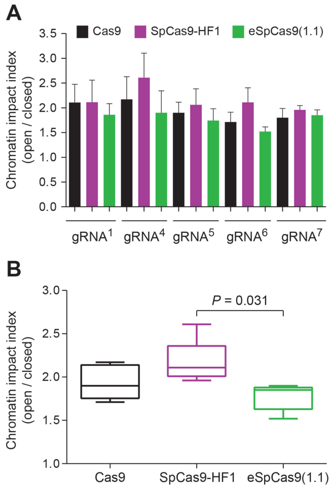
Figure 5. Testing the impact of chromatin conformation on high-specificity Cas9 variants. (A) Screening of CRISPR/Cas9 complexes with different Cas9 proteins in HEK.EGFP TetO:KRAB cells. HEK.EGFP TetO:KRAB cells were incubated in the presence or in the absence of Dox and were subsequently transfected with expression plasmids encoding the indicated CRISPR/Cas9 nuclease components. The chromatin impact index was determined by computing the ratios between EGFP knockout levels measured in the presence versus those determined in the absence of Dox. Error bars indicate mean \pm s.e.m. corresponding to three independent experiments. Ten thousand events, each corresponding to a single viable cell, were measured per sample. (B) Cumulative chromatin impact indexes. Boxplot of the chromatin impact indexes presented in panel A. Whiskers, minimum and maximum. One-way ANOVA compared the experimental groups with a subsequent comparison between groups being done by Bonferroni analysis ( P < 0.05 was considered significant).
