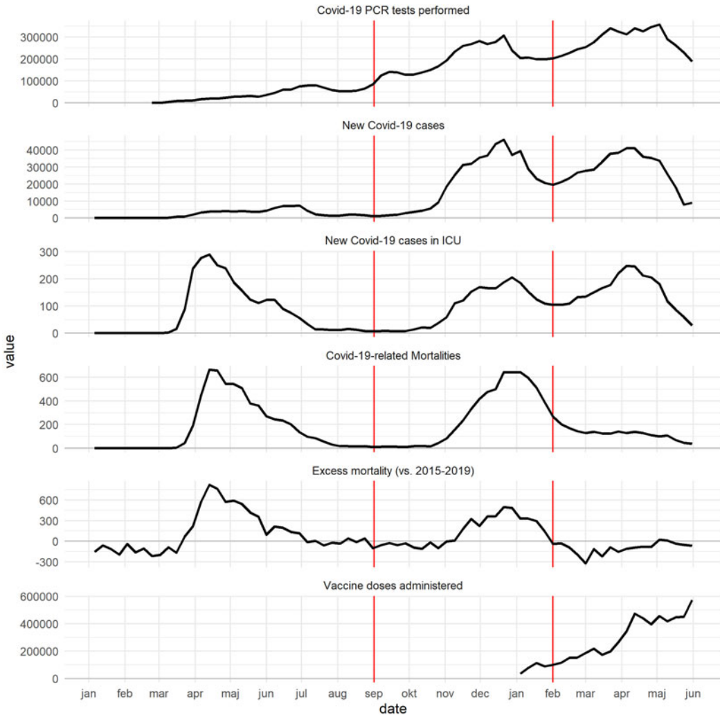
Figure 1. Summary of the weekly data made available by Swedish agencies regarding COVID-19. Red vertical lines denote the delimitation of the three waves as discussed in this paper. Mortality data are truncated to avoid under-reporting of recent weeks. See Supplementary data files stored at Mendelay Data (Spangler, 2021).
