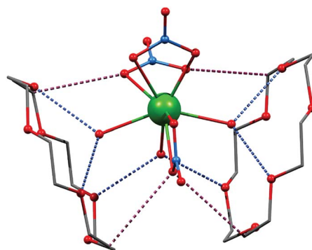
Fig. 1 The molecular structure of 1 showing the second coordination sphere formed by the net of \text{O-H} \cdots \text{O} hydrogen bonds between \text{O-H} atoms of coordinated water and oxygen of crown ether (blue dashed lines) and \text{C-H} \cdots \text{O} (nitrate) contacts (violet dashed line).
