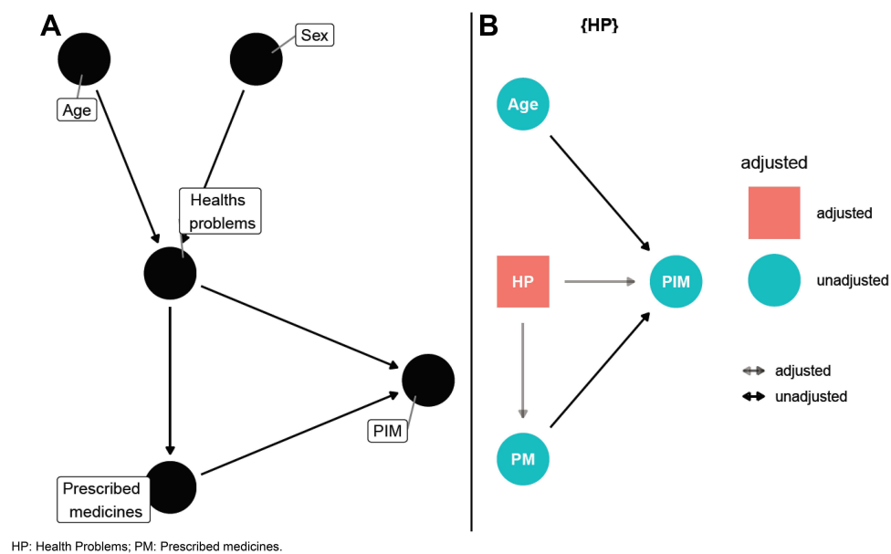
Figure 2 Directed acyclic graphs. Proposed relationship between the different variables (A) and the relationship between the different variables after the appropriate adjustment (B).
