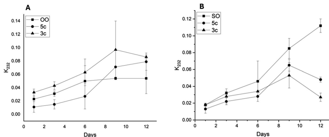
Fig. 9 Evolution of extinction coefficients K_{232} over time of olive oil (A) and sunflower oil (B) supplemented with additives 5c and 3c at 60 °C in the dark. Data points represent mean ( n = 3 ) \pm standard error of the mean.
