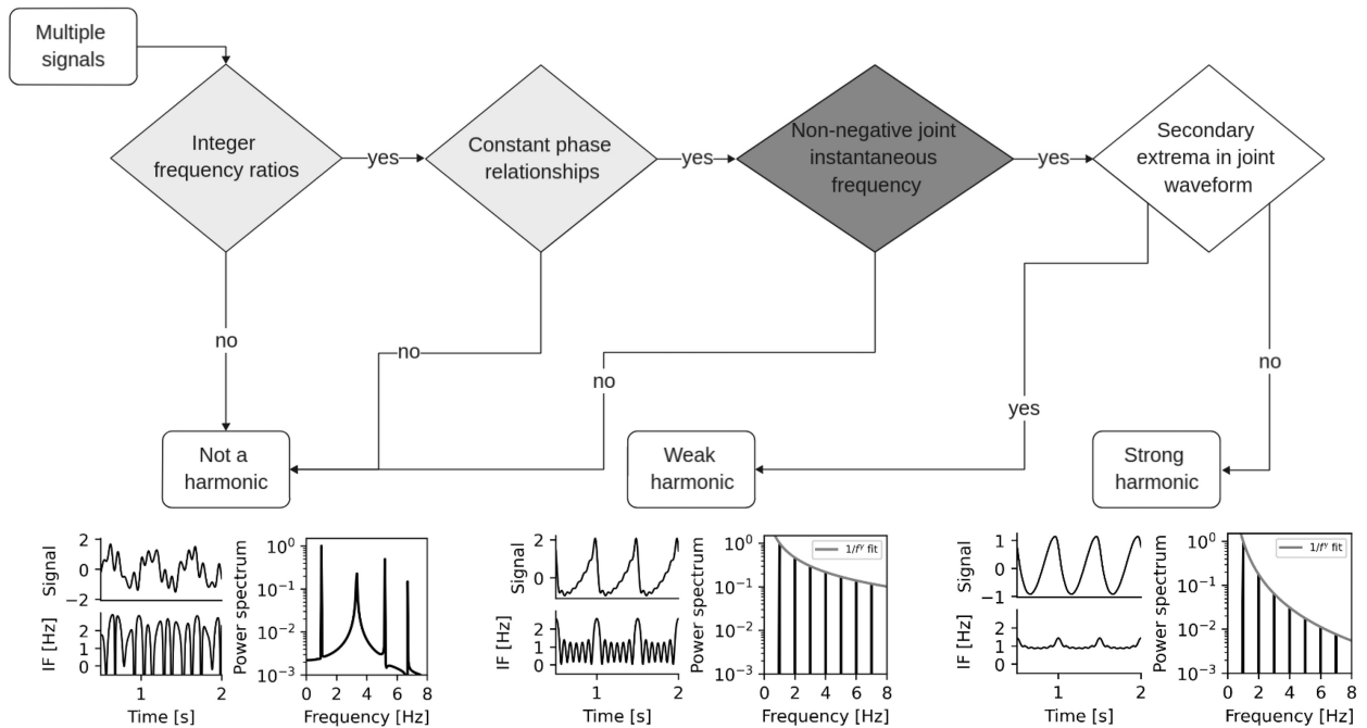
FIGURE 5. Harmonic assessment decision tree. Depending on whether signals meet condition 1 (light grey), condition 2 (dark grey), and how quickly harmonic amplitude falls, the joint signal is either not a harmonic (bottom left, multiple oscillatory processes present and IF sometimes negative), a weak harmonic structure (bottom centre, small secondary extrema present but IF non-negative), or a strong harmonic structure (bottom right, no secondary extrema).
