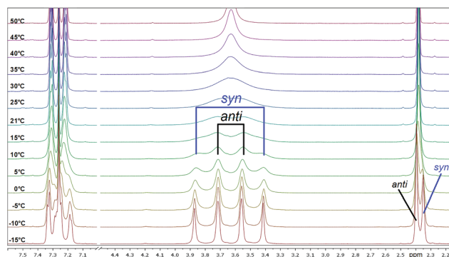
Fig. 4 Temperature-dependent 1 H NMR spectra of 4b measured in CDCl 3 (region of interest from 2.00 to 7.6 ppm is shown).
