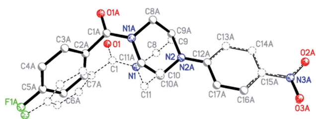
Fig. 10 Superimposition fit of the two conformers, which exist in the ratio of 1 : 1 in the solid-state structure of compound 6d (label A marks the atoms of the second conformer; not all labels shown).
