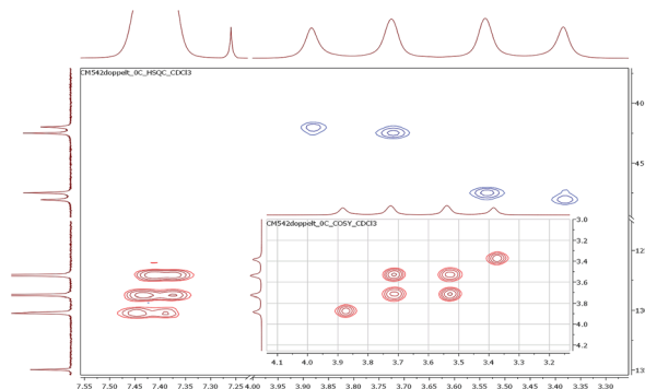
Fig. 2 Part of the 1 H, 13 C-HSQC and H,H-COSY (inset) spectra using the symmetrically disubstituted compound 4a at 0 °C.
