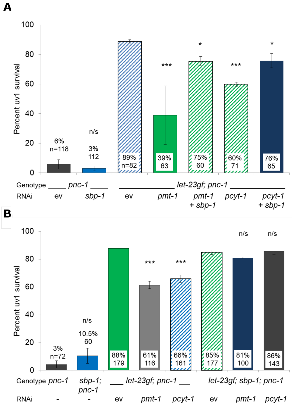
Figure 1: Overactive LET-23 signaling promotes uv1 survival via phosphatidylcholine synthesis and the suppression of SBP-1 activity. A reduction in SBP-1 function by either a) RNAi or b) a sbp-1(ep79) hypomorph (Liang, et al. , 2010) reduces or eliminates the deleterious effect of reduced phosphatidylcholine synthesis from pmt-1 or pcyt-1 RNAi on uv1 cell survival. For a) uv1 cells were counted using an extrachromosomal ida-1::gfp marker, for b) an integrated ida-1::gfp marker was used. ev is RNAi empty vector L4440. Error bars are 1 S.D. with mean percentage uv1 survival, two repeats for a) and three repeats for b) and total number of animals scored. Mean uv1 survival was compared to that of control (ev or single mutant) animals by Fisher's Exact Test; p < 0.05 = * , p < 0.001 = *** , p > 0.05 = n/s .
