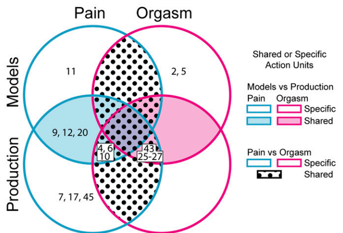
Fig. 5. Comparison of mental representations and productions of facial expressions of pain and orgasm. (A) Classification of facial expression models of pain and orgasm. The color-coded matrix shows the number of facial expression models ( n = 40 total) classified as pain or orgasm based on their highest similarity to real-world productions of facial expressions of pain and orgasm ( n = 14 produced facial expressions in total). Diagonal squares show correct classifications; off-diagonal show incorrect classifications. Warmer colors indicate higher numbers of models; cooler colors indicate lower numbers (see color bar to the right). Exact numbers are shown in each cell. As shown by the diagonal squares, the vast majority of pain and orgasm facial expression models are correctly classified based on the face movements reported in real-world production studies. (B) Comparison of facial expression models of pain and orgasm with real-world productions. The four-set Venn diagram shows the AUs that converge or diverge across the four sets of AUs, reported in facial expression models and produced facial expressions of pain (cyan) and orgasm (magenta). Textured areas show the AUs that are shared between pain and orgasm; shaded areas show the AUs that are shared between models and productions of facial expressions; untextured/unshaded areas show the AUs that are specific to one of the sets (see key to the right).
