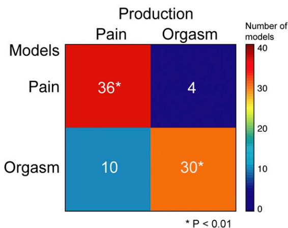
Fig. 5. Comparison of mental representations and productions of facial expressions of pain and orgasm. (A) Classification of facial expression models of pain and orgasm. The color-coded matrix shows the number of facial expression models ( n = 40 total) classified as pain or orgasm based on their highest similarity to real-world productions of facial expressions of pain and orgasm ( n = 14 produced facial expressions in total). Diagonal squares show correct classifications; off-diagonal show incorrect classifications. Warmer colors indicate higher numbers of models; cooler colors indicate lower numbers (see color bar to the right). Exact numbers are shown in each cell. As shown by the diagonal squares, the vast majority of pain and orgasm facial expression models are correctly classified based on the face movements reported in real-world production studies. (B) Comparison of facial expression models of pain and orgasm with real-world productions. The four-set Venn diagram shows the AUs that converge or diverge across the four sets of AUs, reported in facial expression models and produced facial expressions of pain (cyan) and orgasm (magenta). Textured areas show the AUs that are shared between pain and orgasm; shaded areas show the AUs that are shared between models and productions of facial expressions; untextured/unshaded areas show the AUs that are specific to one of the sets (see key to the right).
