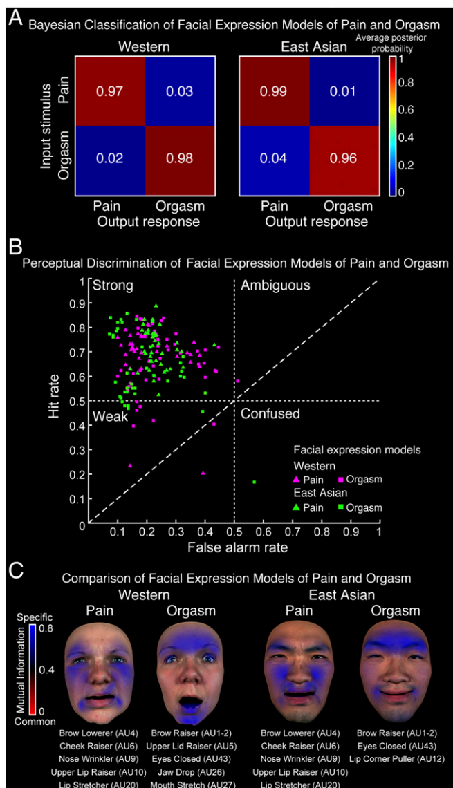
Fig. 3. Distinctiveness of the facial expression models of pain and orgasm in each culture. (A) Bayesian classification of facial expression models of pain and orgasm. Color-coded matrices show for each culture the average posterior probability that a facial expression model of pain or orgasm (input stimulus) is classified as pain or orgasm (output response). Red shows high posterior probability of classification; blue indicates low posterior probability (see color bar to the right). Exact values are shown in each square. Diagonal squares show correct classifications; off-diagonal squares show incorrect classifications. The red-colored diagonal squares show that in each culture the facial expression models of pain and orgasm are discriminated with high accuracy. (B) Perceptual discrimination of facial expression models of pain and orgasm. Each color-coded shape represents an individual observer facial expression model ( n = 40 per culture) plotted according to its hit rate and its false alarm rate (i.e., d -prime value, which is a measure of perceptual discrimination). Magenta points represent Western models, and green represents East Asian models; triangles represent pain, and squares represent orgasm (see legend in the bottom right). The four quadrants (delimited by dashed lines) indicate the different response types based on hit and false alarm rates (see labels in each quadrant). The diagonal dashed line represents an equal rate of hits and false alarms. The distribution of the data points in the upper left-hand quadrant shows that the vast majority of facial expression models from both cultures are discriminated well with virtually no instances of ambiguity or confusion. (C) Comparison of facial expression models of pain and orgasm. To objectively identify which face movements (i.e., AUs) are specific to or common across pain and orgasm in each culture, we used mutual information ( Methods, Comparison of the Facial Expression Models of Pain and Orgasm ). For each culture, blue coloring on the face
