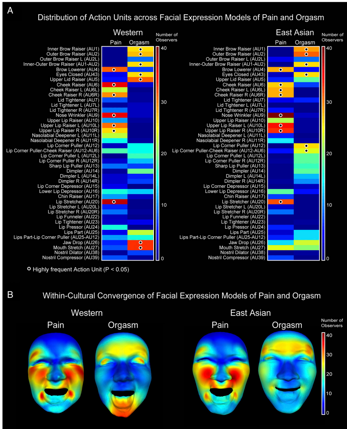
Fig. 2. Distribution of action units across facial expression models of pain and orgasm and their convergence across observers within each culture. (A) Distribution of AUs across facial expression models of pain and orgasm. For each culture—Western (Left) and East Asian (Right)—and pain and orgasm separately, the color-coded matrix shows the number of individual observer facial expression models (maximum 40) with each AU (see labels on the left). Warmer colors indicate more observers; cooler colors indicate fewer observers (see color bar on the right). A black dot indicates the AUs that are highly frequent (one-tailed, P < 0.05 ) across all individual observer models as determined using a Monte Carlo simulation method ( SI Appendix, Highly Frequent Action Units ). (B) Within-culture convergence of facial expression models of pain and orgasm. Color-coded face maps show for each culture and affective state the number of individual observer facial expression models with each AU using the same color coding as in A.
