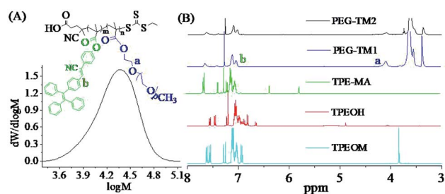
Fig. 2 (A) The GPC trace of PEG-TM1 (THF) ( M_n = 25\,000 , \text{PDI} = 1.30 ); (B) ^1\text{H NMR} spectra ( \text{CDCl}_3 ) of TPEOM, TPEOH, fluorescent monomer TPMA and fluorescent polymers PEG-TM.
