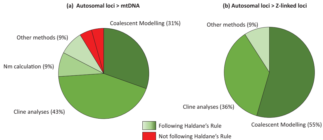
Figure 2. The literature review revealed that most studies reported introgression patterns in line with Haldane's Rule, with (a) higher introgression of autosomal loci compared to mtDNA, and (b) higher introgression of autosomal loci compared to Z-linked loci. The studies used a variety of methods to infer patterns of introgression.
