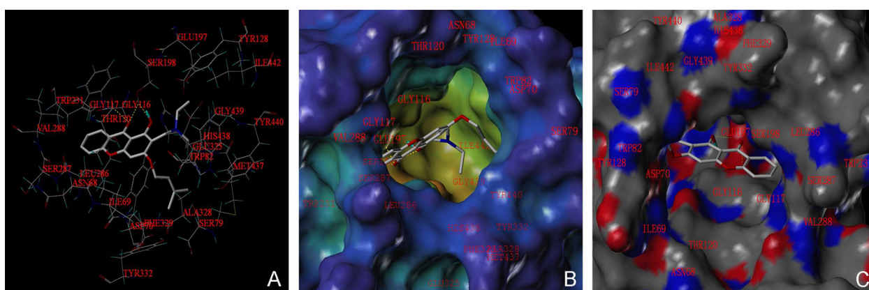
Figure 6 The binding mode research of compound 4b on BuChE by docking simulations. (A) The binding interactions with selected residues of the active site for compound 4b. (B) The MOLCAD surfaces displayed with cavity depth potential of the binding pocket. (C) The MOLCAD hydrogen bonding surfaces of the binding pocket.
