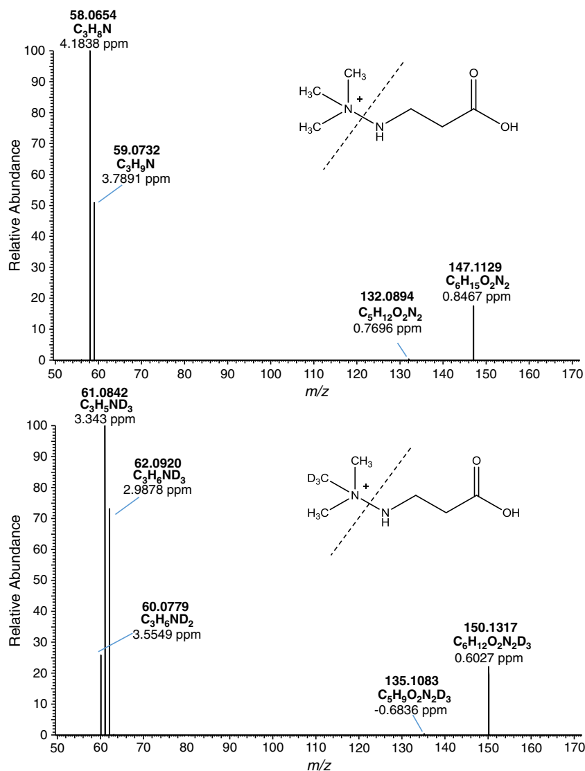
Figure 2. Product ion t-HCD mass spectra of the permanent positively charged Mildronate and Mildronate- D_3 (IS) precursor ions at m/z 147.1129 and m/z 150.1317 measured in a spiked urine sample by means of high resolution/high accuracy mass spectrometry using a Q Exactive hybrid quadrupole-orbitrap ® mass spectrometer (17,500 FWHM, NCE: 50%).
