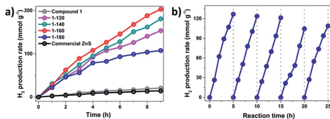
Fig. 6 (a) Plots of photocatalytic \text{H}_2 evolution amount of 1, 1-120, 1-140, 1-160, 1-180 and commercial ZnS vs. irradiation time. (b) Cycle runs of photocatalytic \text{H}_2 production over the 1-160 photocatalyst.
