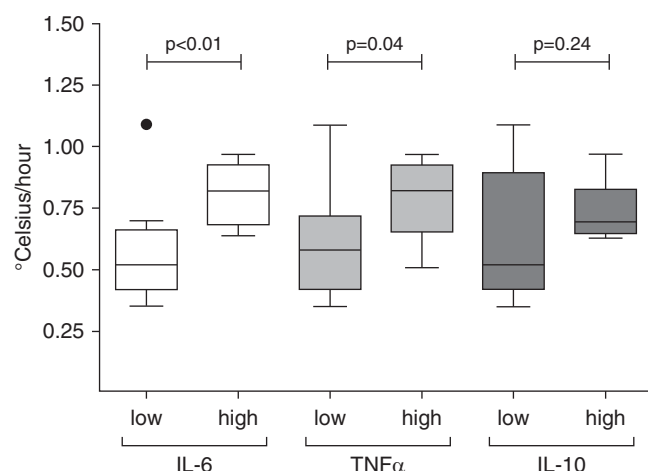
Figure 1. Slope of the temperature increase ( \text{Temp}_{\text{slope}} ) after endotoxin administration for subjects with low and high peak levels of IL-6, \text{TNF}\alpha (tumor necrosis factor \alpha ), and IL-10. Data are presented as box-and-whisker plots (Tukey).
