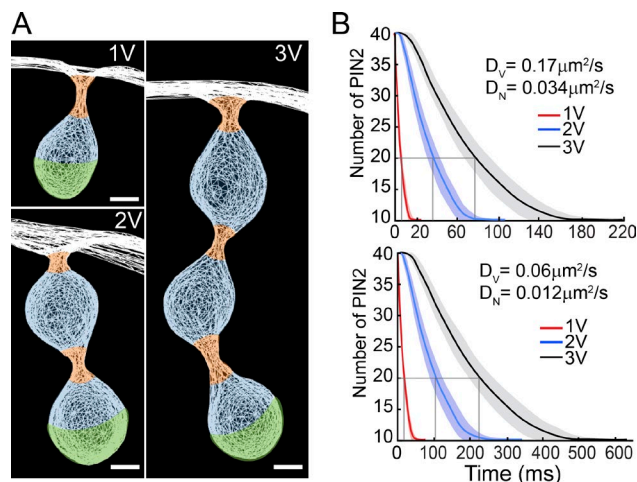
Figure 4. Simulation of cargo escape in concatenated ILV geometries. (A) Geometries derived from electron tomograms of plant MVEs used for the cargo diffusion simulations depicted in B. Green indicates the lower ILV hemisphere, where the PIN2 molecules were placed to start the simulation, orange indicates the ILV bud neck and interconnecting membrane bridges, blue indicates the rest of the internalized membrane, and white indicates the endosomal limiting membrane. Bars, 10 nm. (B) Simulated escape times of 40 PIN2 particles placed on the lower hemisphere of the ILV bud using two D values ( 0.06 and 0.17 \mu\text{m}^2/\text{s} ). The colored lines indicate the mean numbers of remaining cargo over time calculated from >300 simulations, and the shaded regions correspond with the SD. Gray vertical lines indicate the mean times required for 50% of the PIN2 particle to escape the ILV bud. Simulations were run incorporating volume exclusion and a fivefold decrease in D when PIN2 particles entered neck or bridge regions (orange in A).
