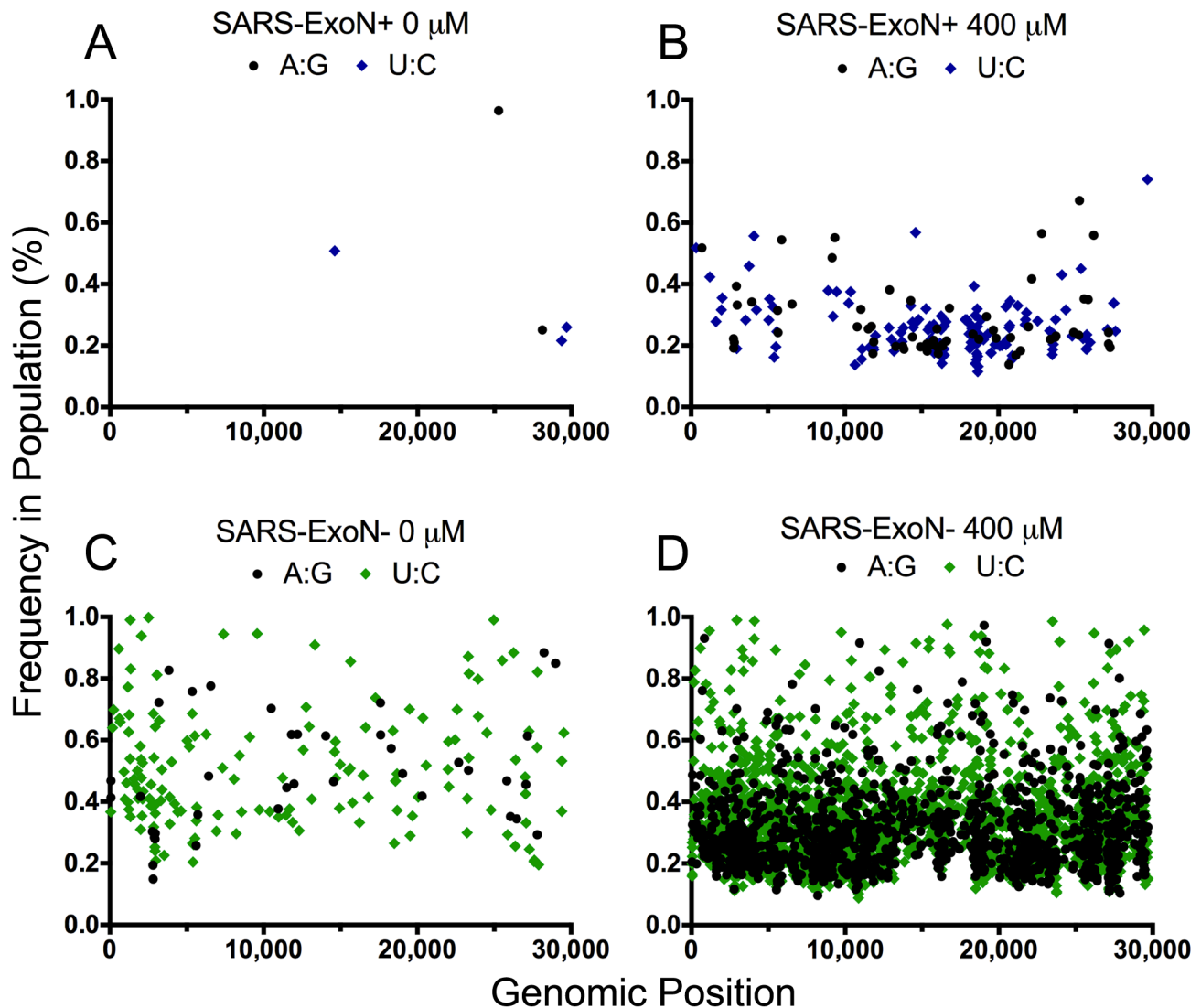
Figure 5. 5-FU-mediated U:C and A:G transitions are distributed across the CoV genome at low frequency. (A) and (B) The genomic distribution of low frequency statistically significant U:C and A:G variants within the SARS-ExoN+ population following treatment with 0 or 400 \mu\text{M} 5-FU. (C) and (D) Same as in A and B except for the SARS-ExoN- population. For all panels, SARS-ExoN+ viruses are shown in blue, and SARS-ExoN- viruses are shown in green. U:C transitions are denoted by a diamond, whereas A:G transitions are plotted as circles. doi:10.1371/journal.ppat.1003565.g005
