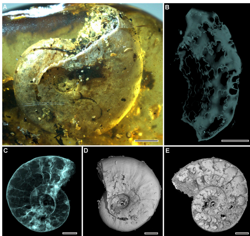
Fig. 2. Ammonite Puzosia (Bhimaites) Matsumoto. (A) Lateral view under light microscopy. (B) Flattened sutures reconstructed by microtomography. (C) Microtomographic reconstruction, apparent view. (D) Microtomographic reconstruction, surface rendering; (E) Microtomographic reconstruction, virtual section. (Scale bars, 2 mm.)
