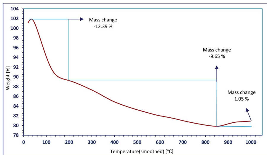
Fig. 6 TGA curve of the Ni/ \text{SO}_3\text{H}@ zeolite-Y.
