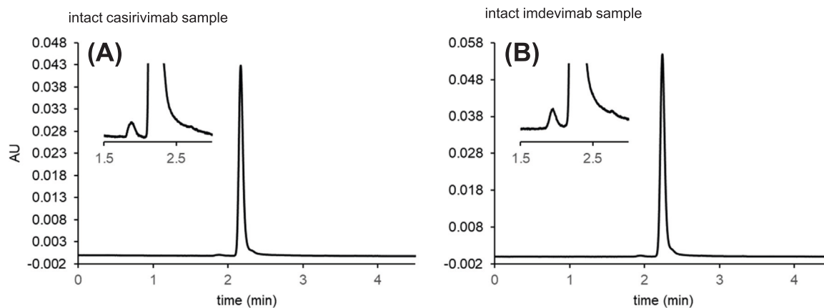
Fig. 6. Optimized separation conditions for SEC analysis of intact Casirivimab (A) and Imdevimab (B). Column: 4.6 \times 150 mm, flow rate F = 0.5 mL/min; analysis time: 4.5 min; T = 25 °C; injected volume: 1 \mu L; UV detection at 280 nm. MP: 1 \times PBS buffer, pH = 7.4.
