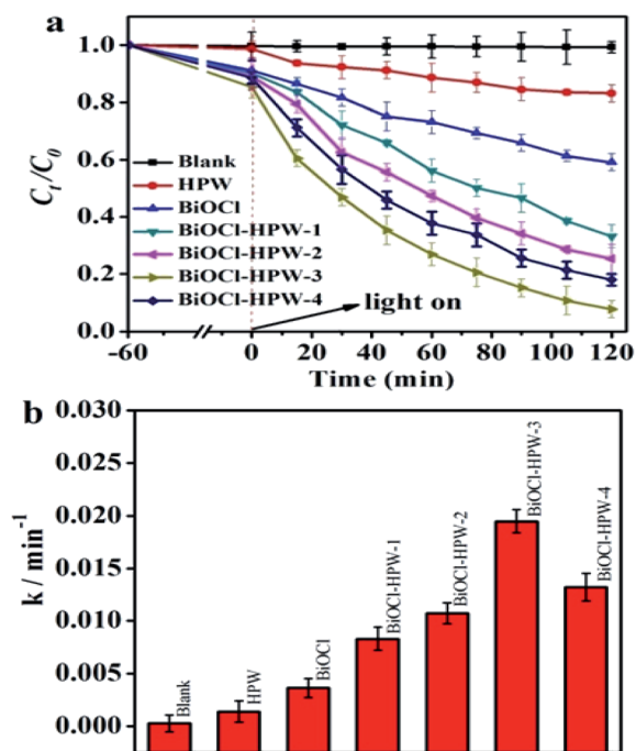
Fig. 3 The photocatalytic efficiency (a) and the apparent rate constant (b) of BiOCl, HPW and BiOCl-HPW-3. The photo-catalyst concentration was 0.2 mg mL -1 and TC concentration was 10 mg L -1 .
