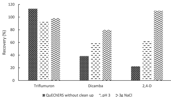
Fig. 2. Recoveries results obtained for triflururon, dicamba and 2,4-D with the methodologies assayed.
