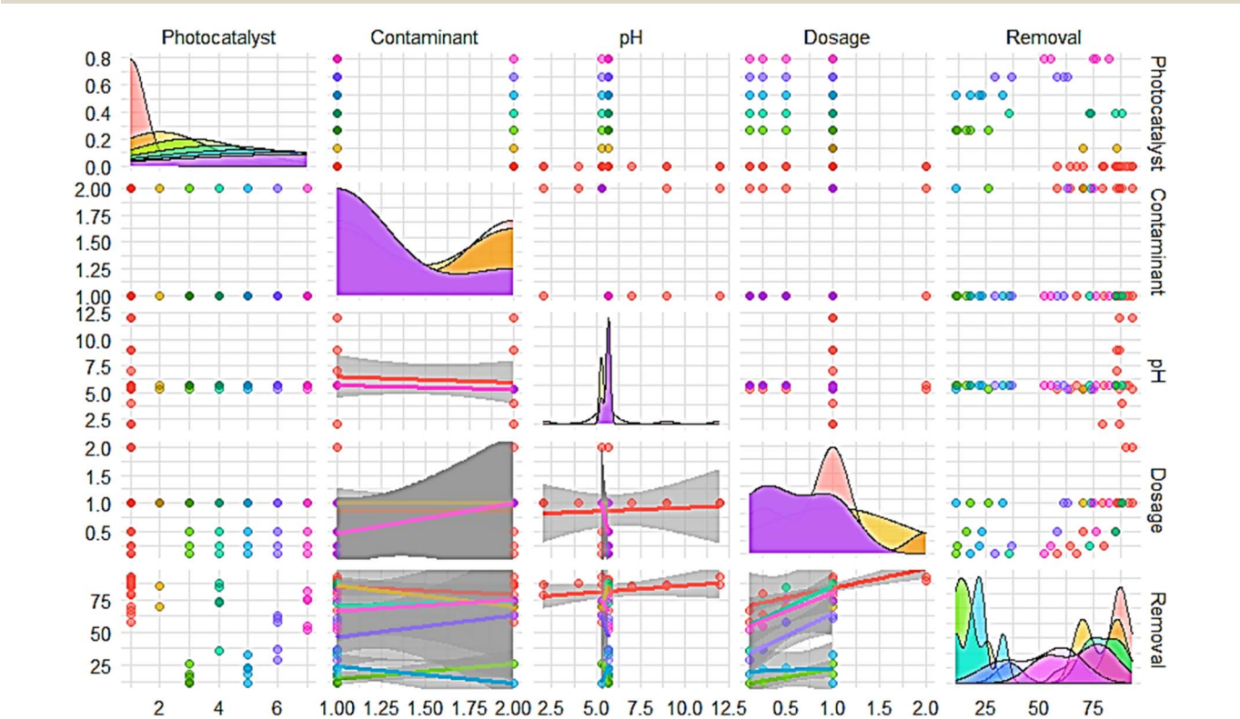
Fig. 12 Scatter matrix plot representing the distribution and trends present in the data set.
