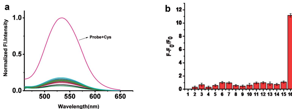
Fig. 3 (a) The fluorescence spectra of probe 1 (5 \mu\text{M} ) toward Cys (10 \mu\text{M} ), Hcy, GSH and various amino acids (10 \mu\text{M} ) in \text{H}_2\text{O} : \text{ethanol} = 8 : 2 (v/v), pH = 7.4, 10 mM PBS at room temperature: the inset shows the fluorescence of various solution under the Handhold UV Lamps (365 nm). (b) Fluorescence intensity changes at 525 nm. (1) Probe 1 (2) L-Leu (3) Ala (4) Trp (5) L-Met (6) Val (7) Thr (8) Tyr (9) D-Met (10) Ser (11) Glu (12) Phe (13) D-Leu (14) GSH (15) Hcy (16) Cys. Excitation wavelength is 400 nm, excitation and emission slit widths are 5 nm and 5 nm. Each spectrum was acquired 40 min after various analytes addition at room temperature.
