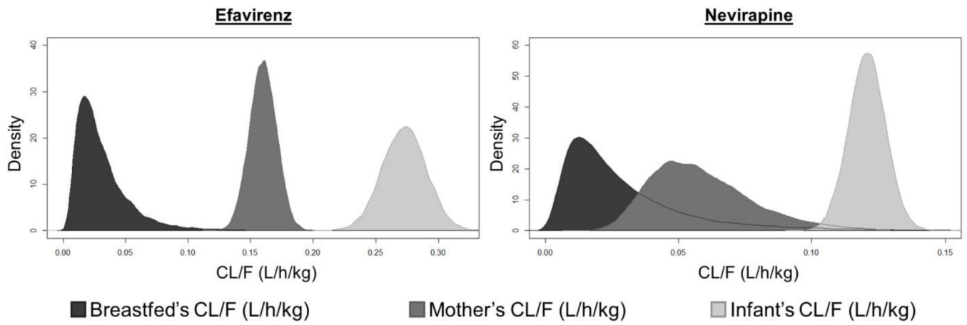
Fig. 3. Distribution of simulated breastfed newborns', mothers' and infants' apparent clearances
