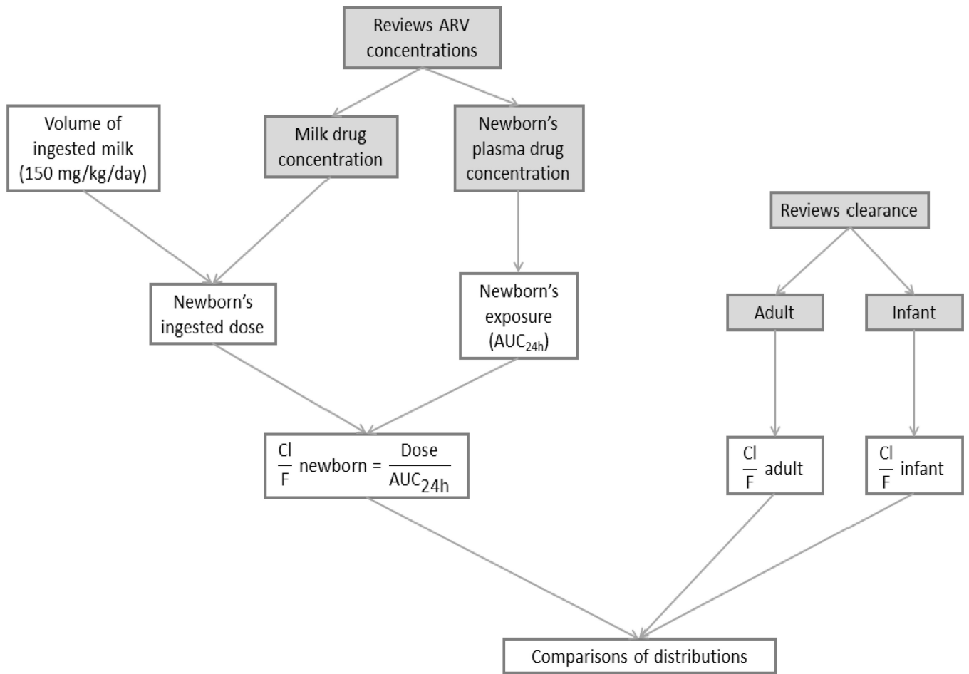
Fig. 1. Estimation of newborn's and mother's apparent clearance
